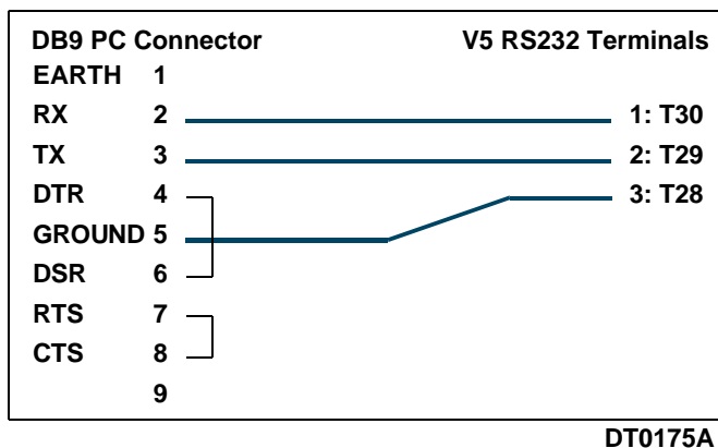
Figure 2.2: RS232 Wiring.
